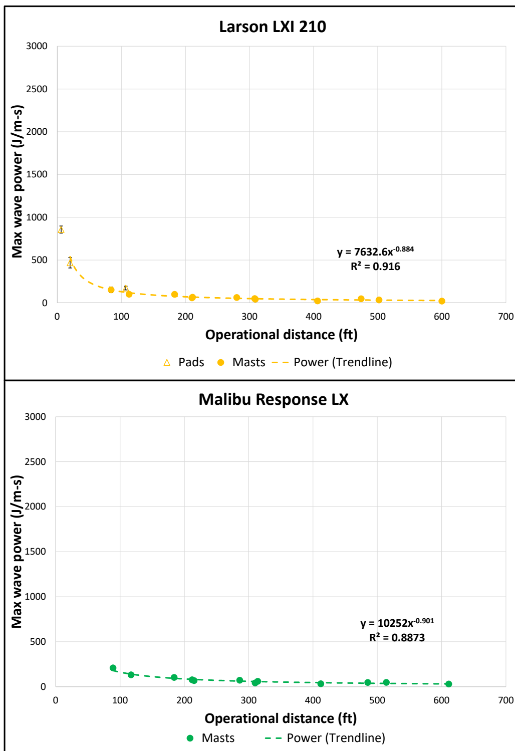
Figure 19. Maximum wave power as a function of wave propagation distance for the two non-wakesurf boats tested under Condition 1a. There are no data for the Pads for the Malibu Response LX due to technical issues with the ADCP on test day. Data points less than one boat length from the track line were not included in the regression analysis.
