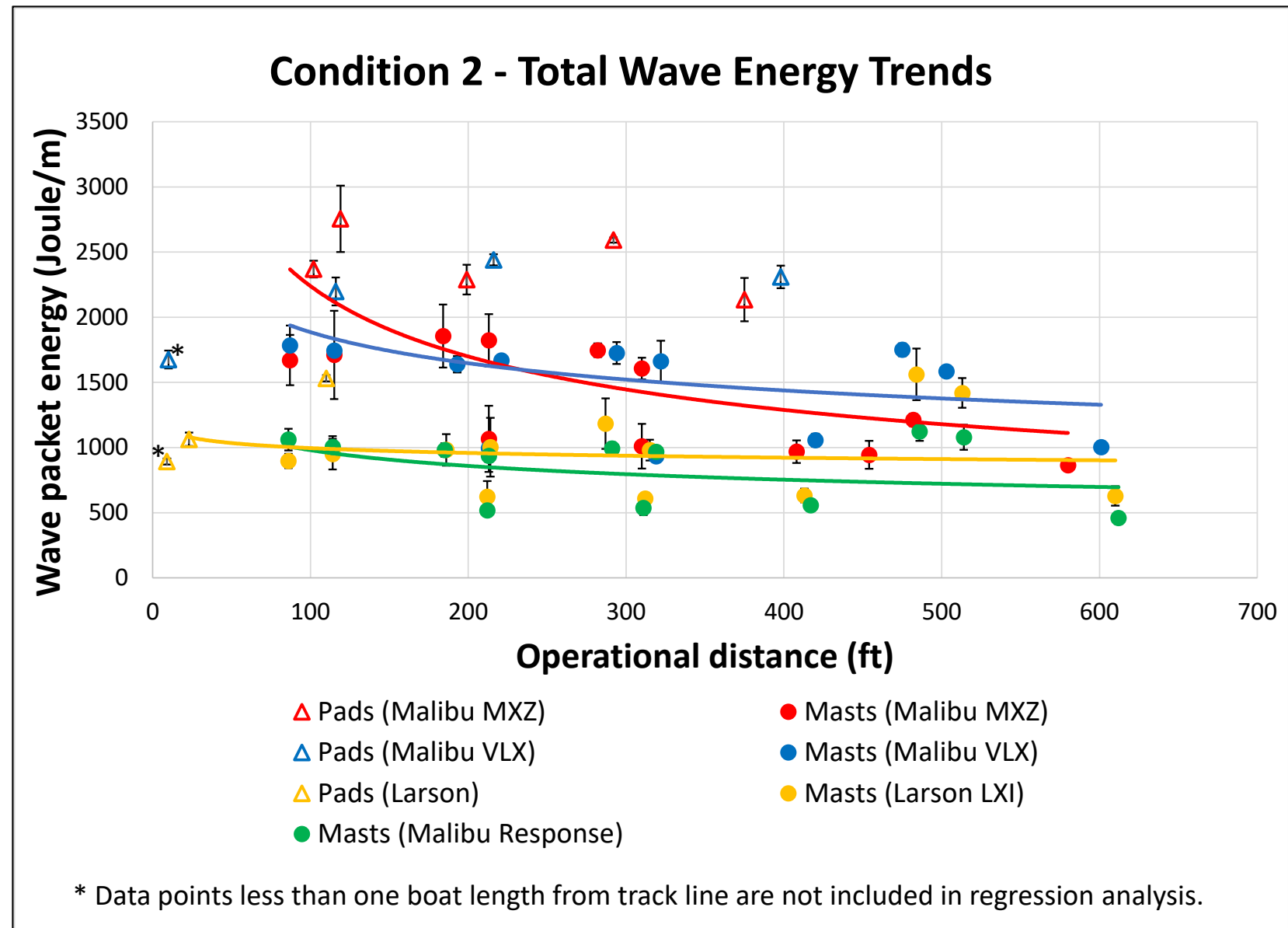
Figure 27. Condition 2 trendlines for the four test boats showing total wave energy over operational distance.
