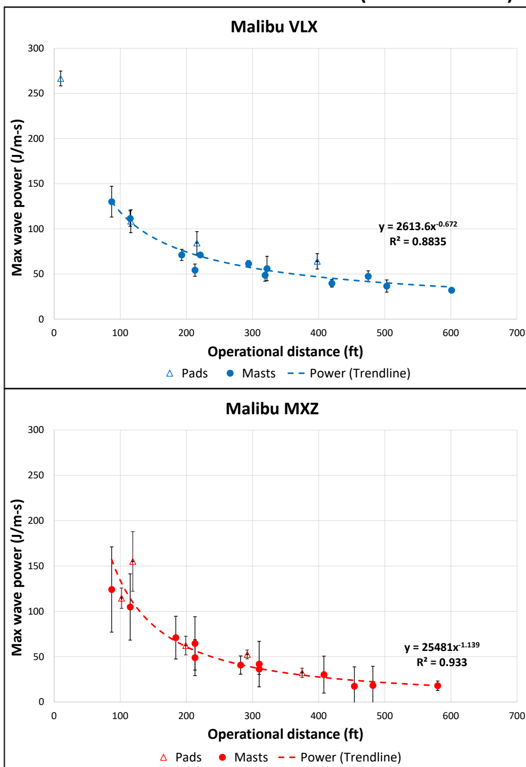
Figure 29. Maximum wave power as a function of operational distance for the two wakesurf boats tested under Condition 2. The Pad data at distances less than 100 ft for the Malibu MXZ were noisy and thus eliminated from this analysis. Data points less than one boat length from the track line were not included in the regression analysis.
