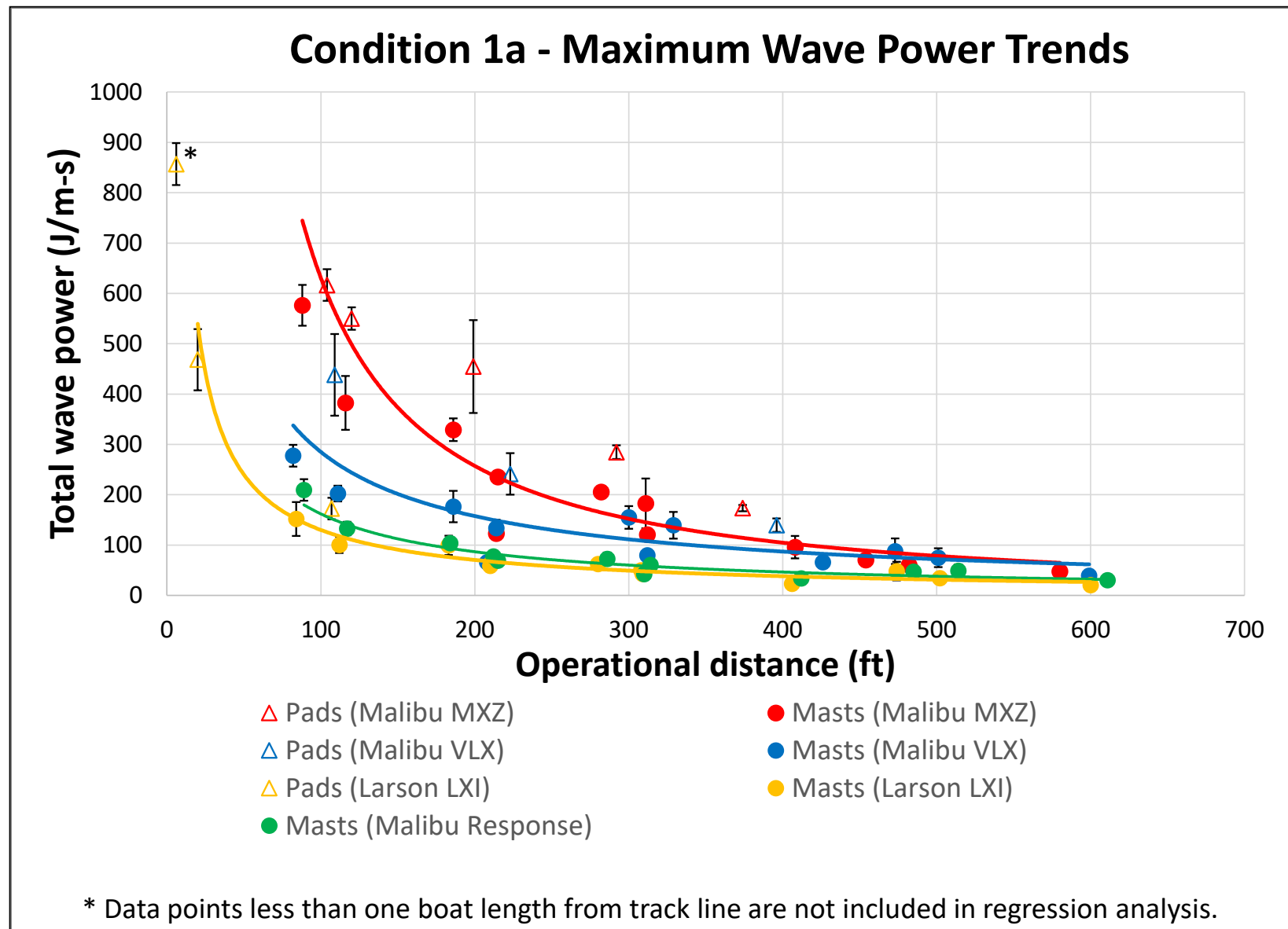
Figure 21. Condition 1a trendlines for the four test boats showing maximum wave power over operational distance.
