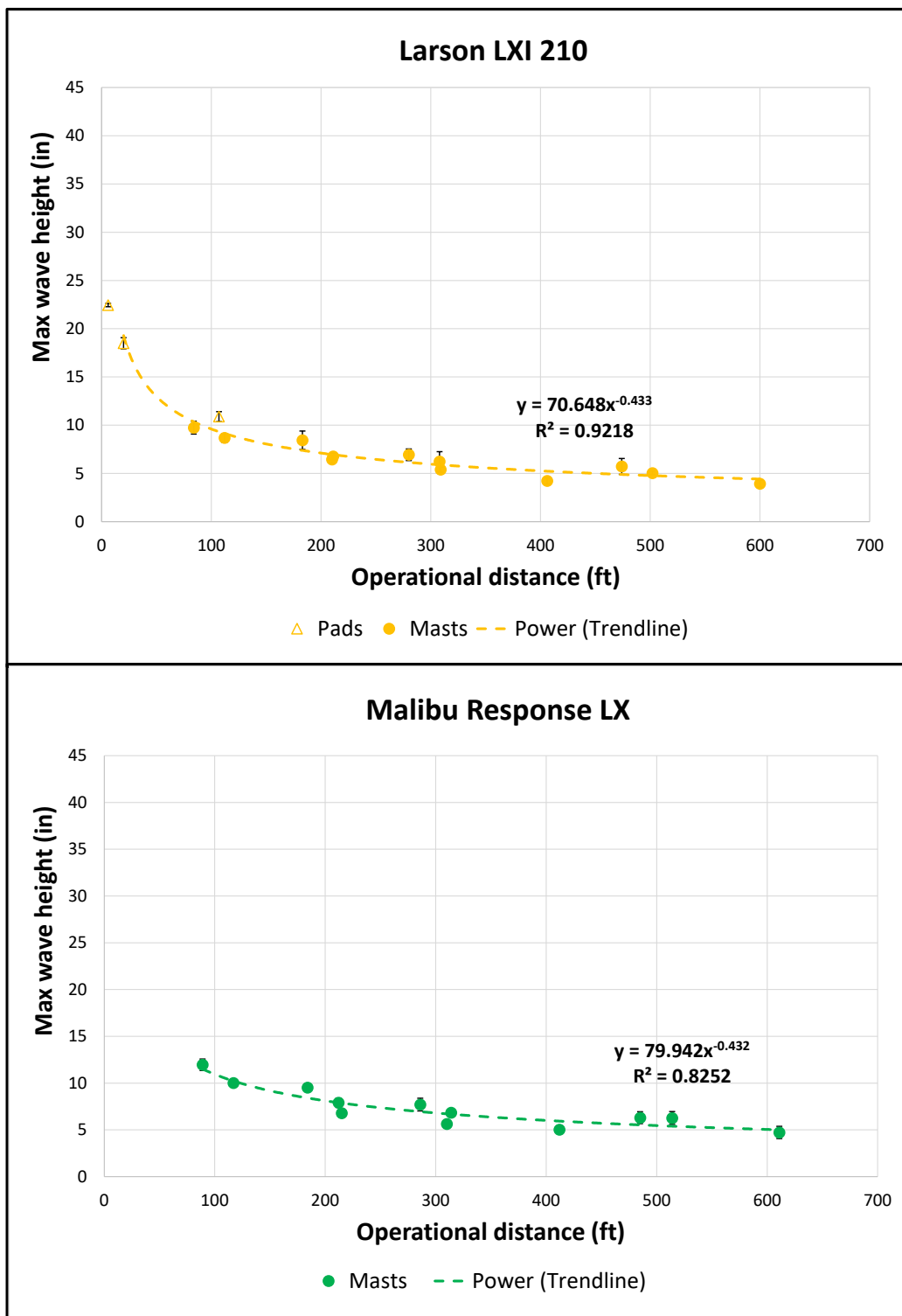
Figure 13. Maximum wave height as a function of distance for the two non-wakesurf boats tested under Condition 1a. The error bars represent the standard deviation. There are no data for the Pads for the Malibu Response LX due to technical issues with the ADCP on test day. Data points less than one boat length from the track line were not included in the regression analysis.
